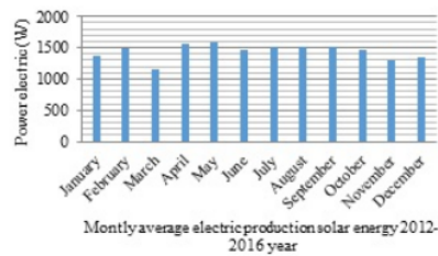
Fig. 6. Monthly production solar energy for 2012-2016
